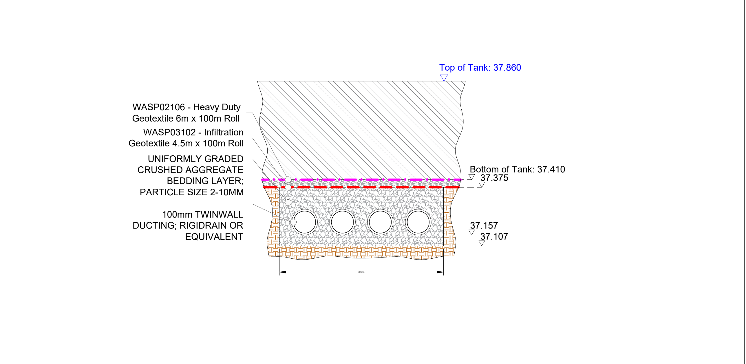
Services Ducting Section (Scale: 1:10)
