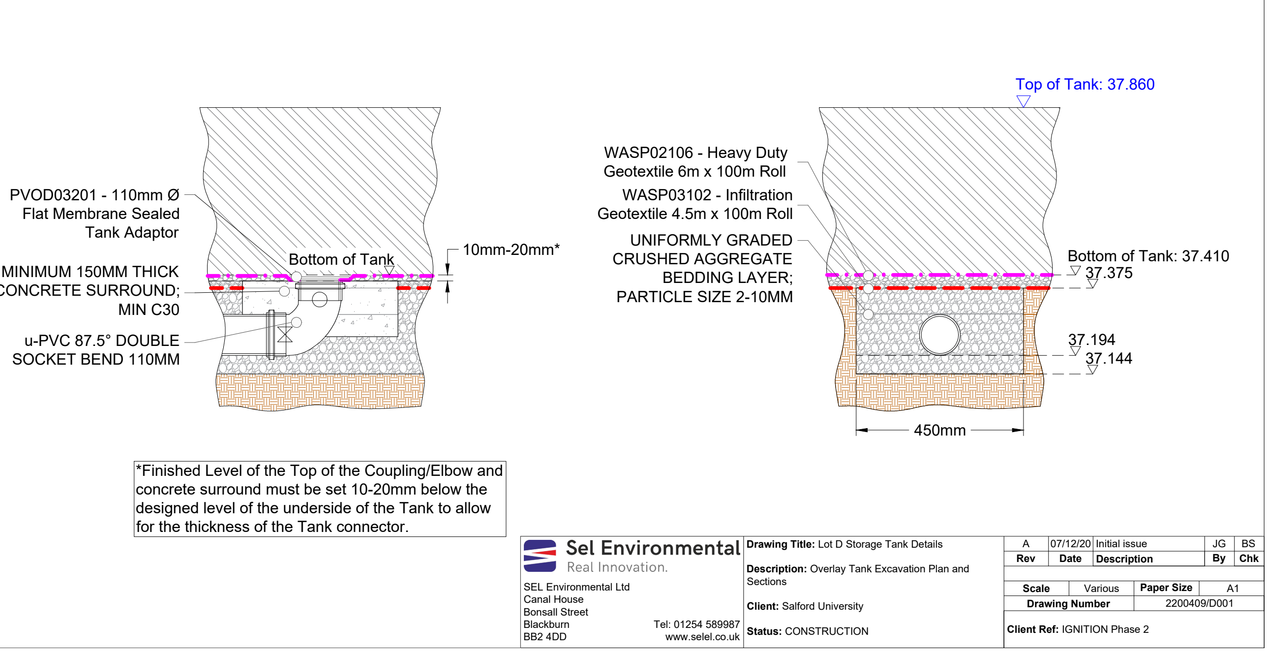
Tank Connection Pipe Section (Scale: 1:10)
