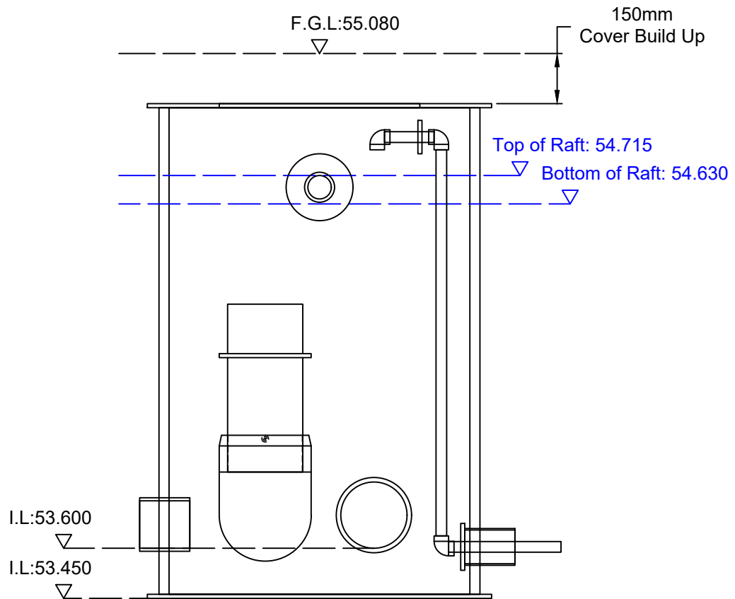
Section B-B CwC Chamber
