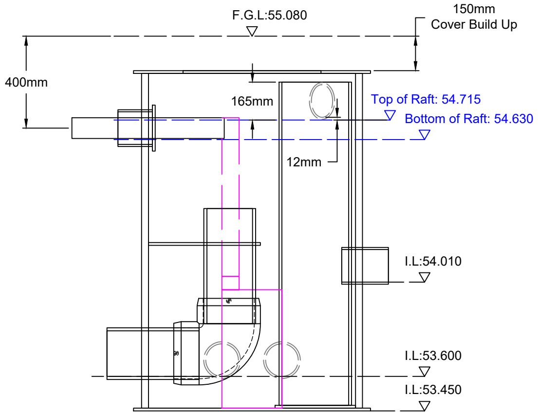
Section A-A CwC Chamber
